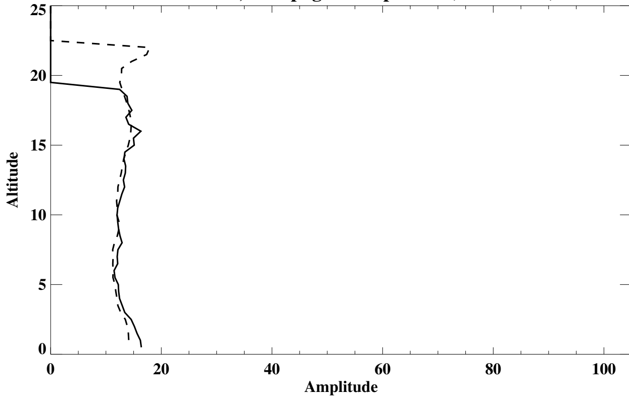
San Cristobal, Galapagos' Amplitude (% of mean)
