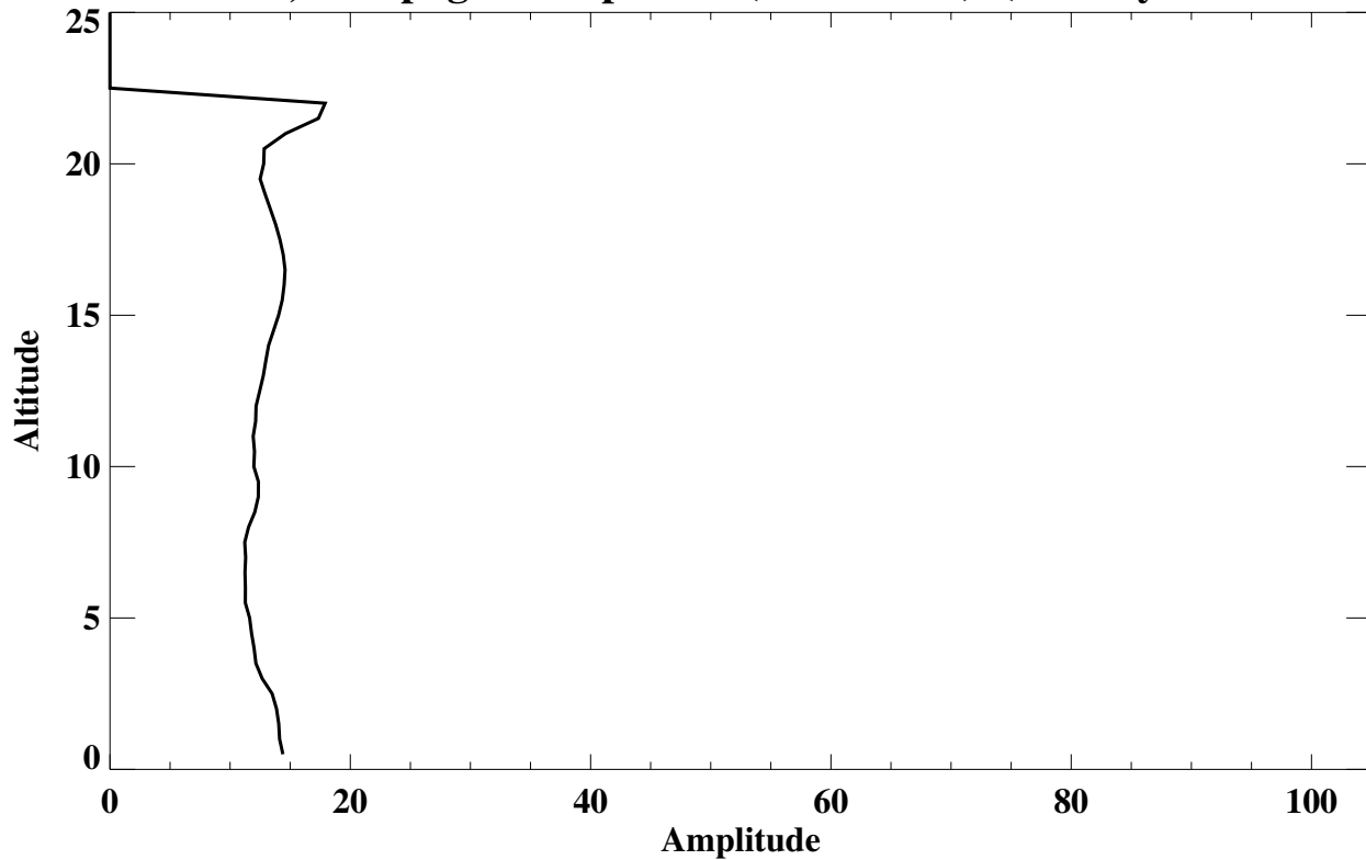
San Cristobal, Galapagos' Amplitude (% of mean) (Gravity Wave Lamina)
