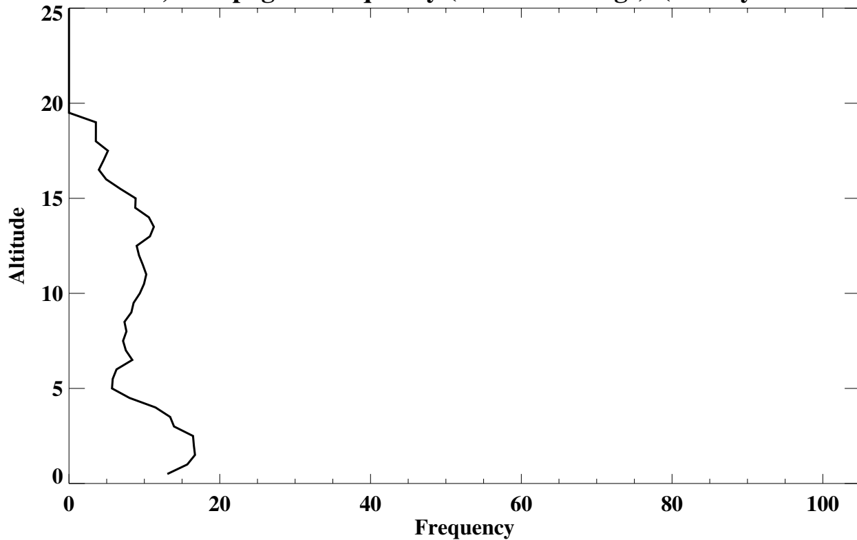
San Cristobal, Galapagos' Frequency (% of soundings) (Rossby wave Lamina)
