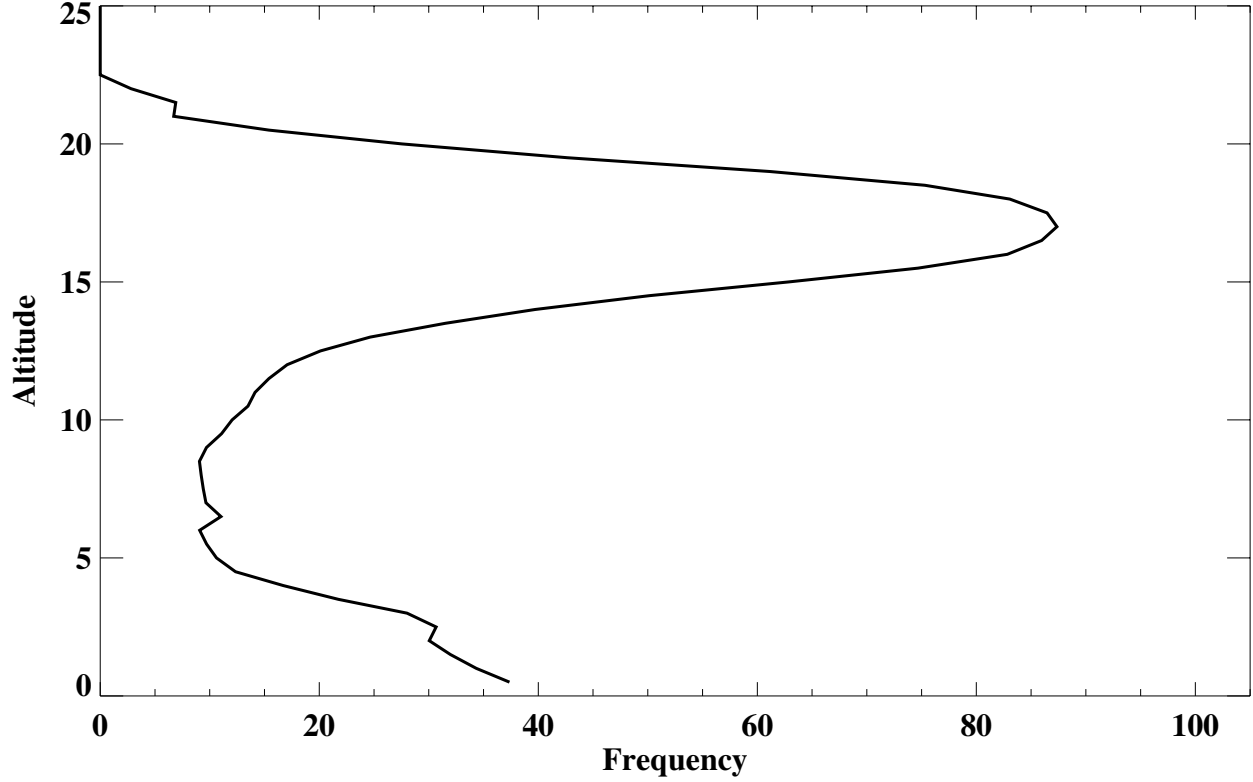
San Cristobal, Galapagos' Frequency (% of soundings) (Total Lamina)
