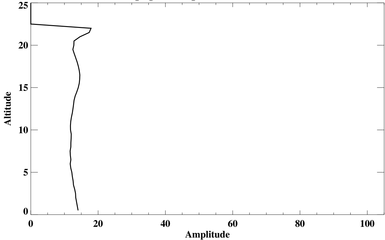
San Cristobal, Galapagos' Amplitude (% of mean) (Total Lamina)
