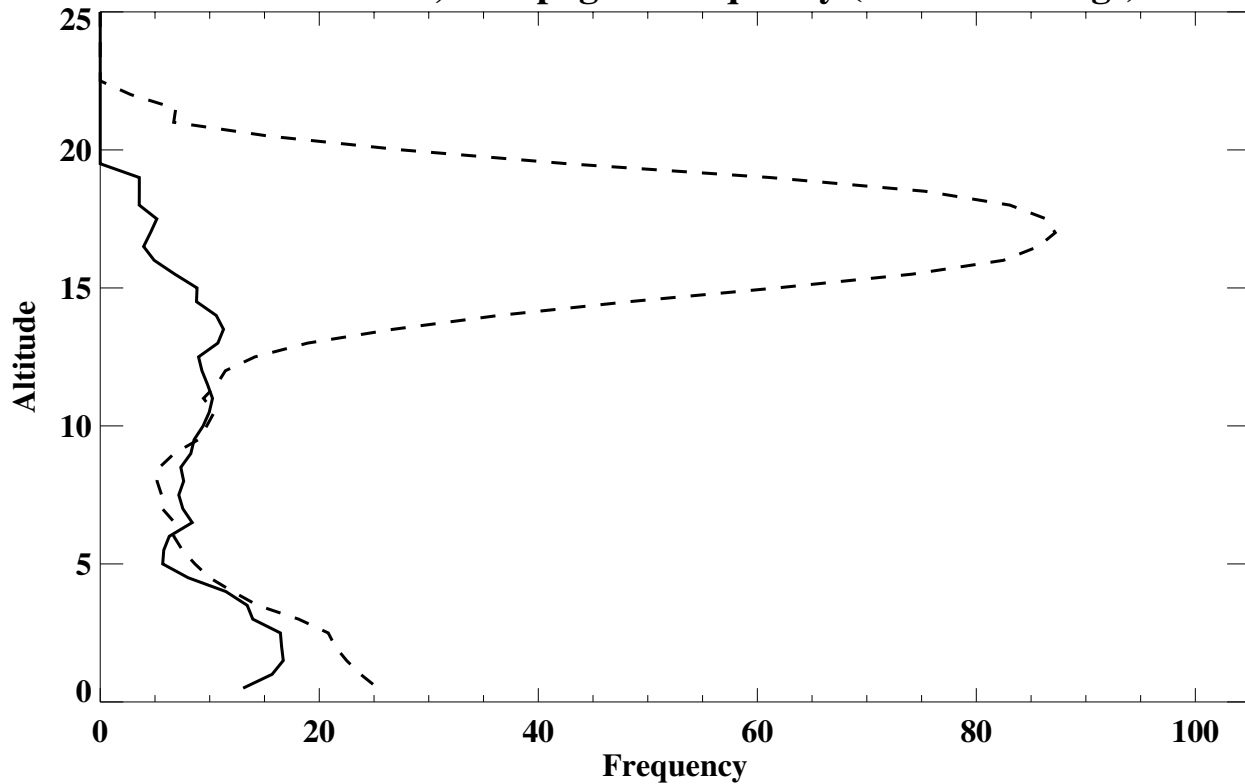
San Cristobal, Galapagos' Frequency (% of soundings)
