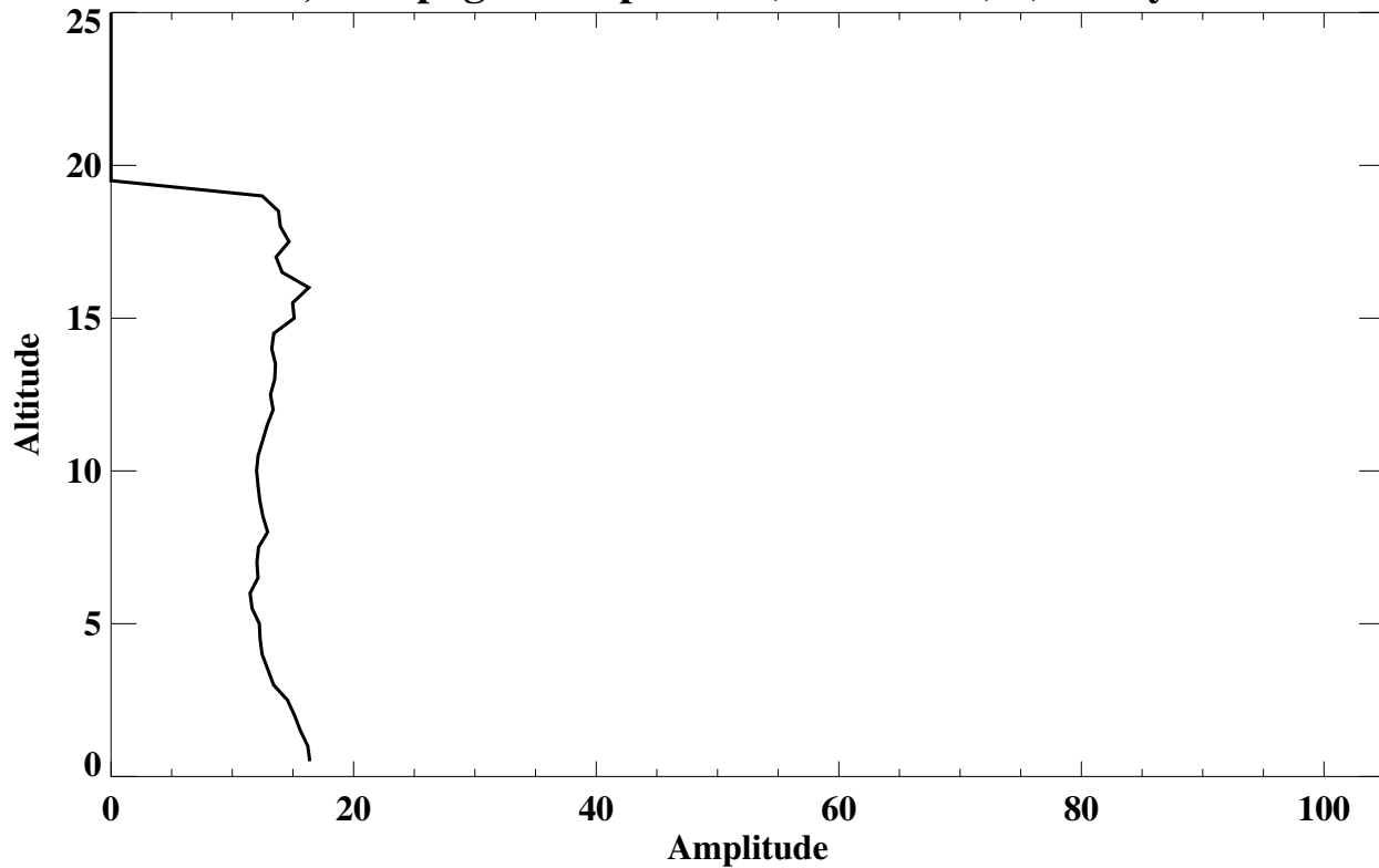
San Cristobal, Galapagos' Amplitude (% of mean) (Rossby wave Lamina)
