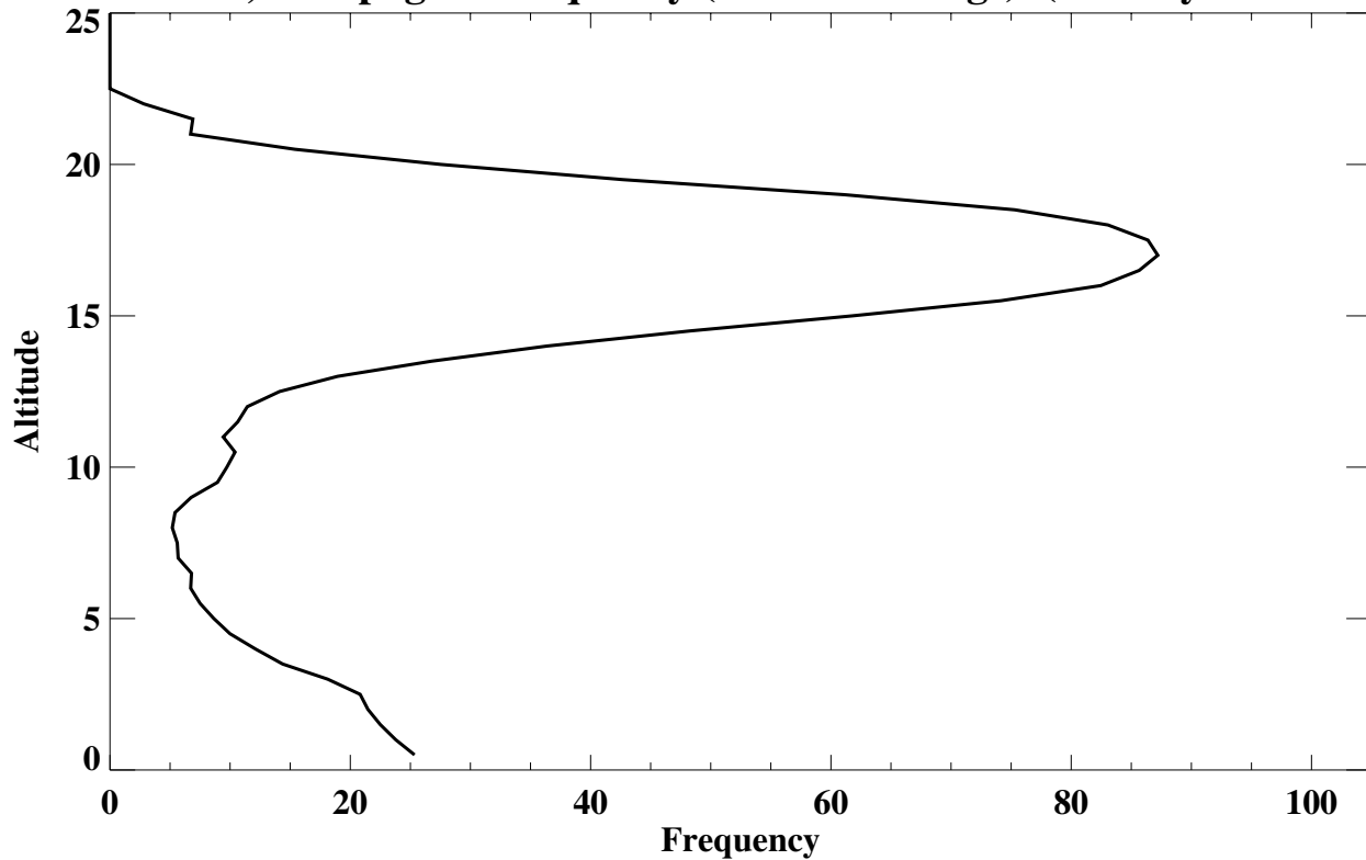
San Cristobal, Galapagos' Frequency (% of soundings) (Gravity Wave Lamina)
