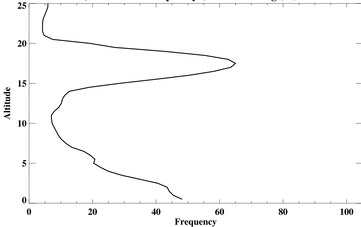
Paramaribo, Suriname' Frequency (% of soundings) (Total Lamina)
