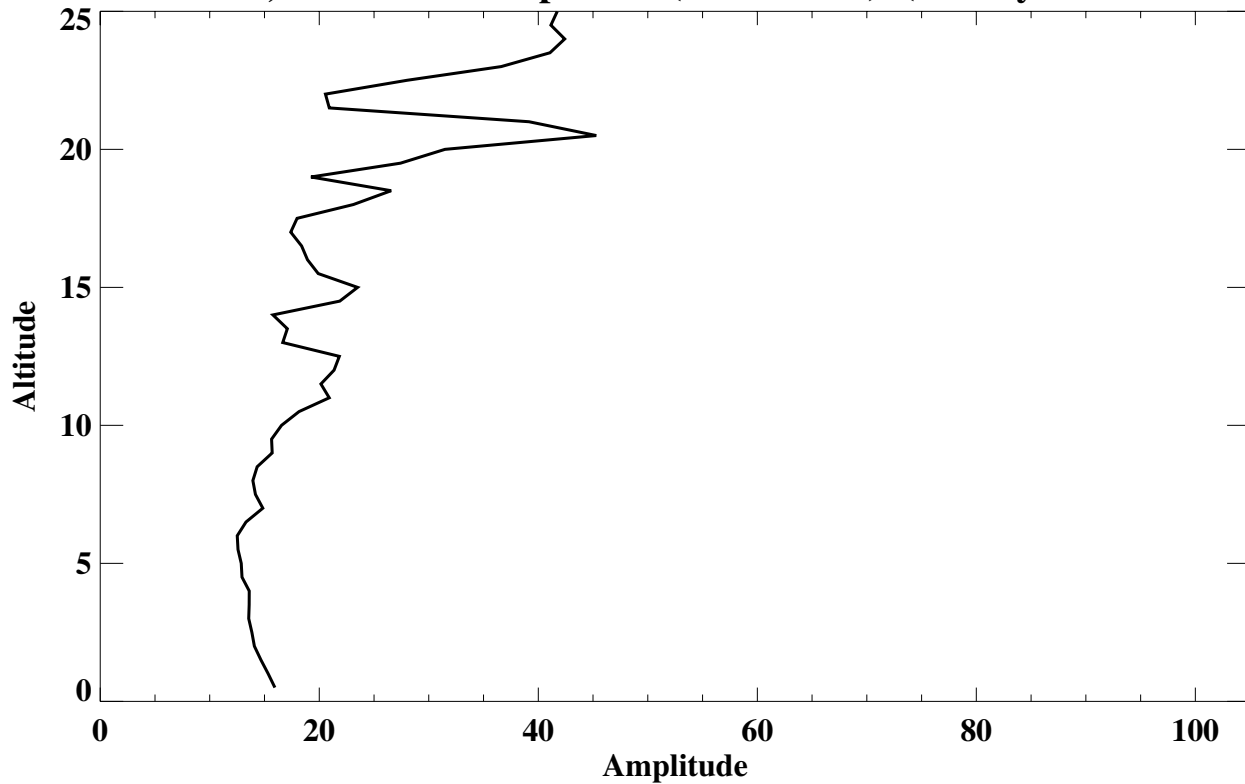
Paramaribo, Suriname' Amplitude (% of mean) (Rossby wave Lamina)
