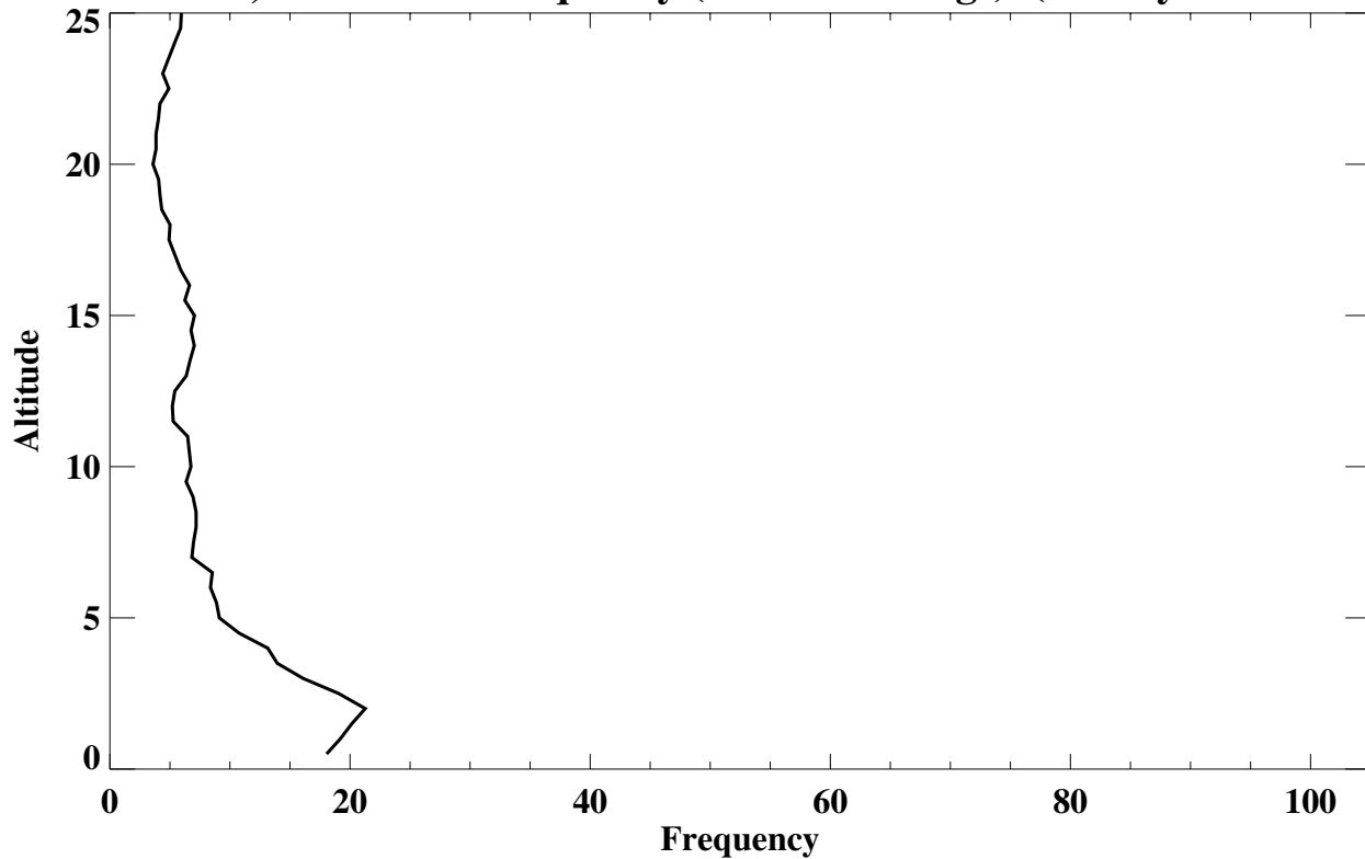
Paramaribo, Suriname' Frequency (% of soundings) (Rossby wave Lamina)
