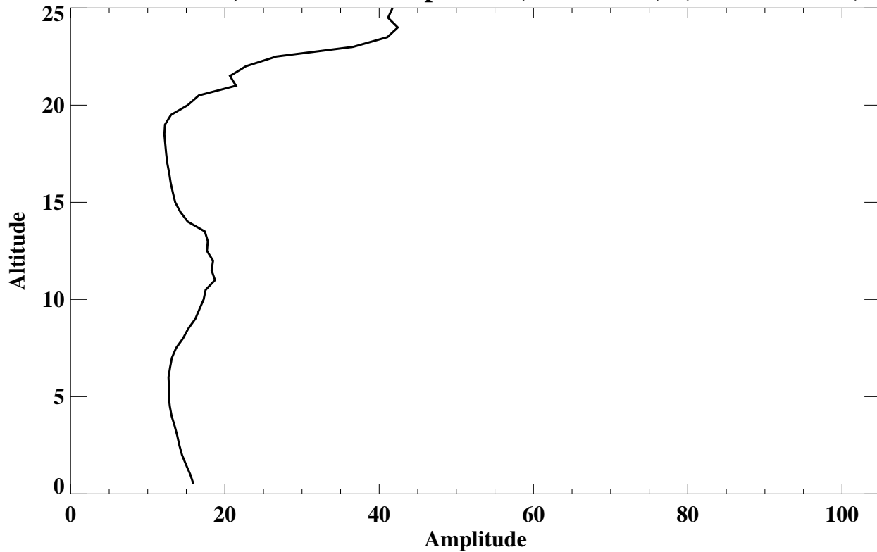
Paramaribo, Suriname' Amplitude (% of mean) (Total Lamina)
