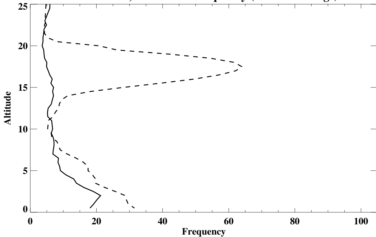
Paramaribo, Suriname' Frequency (% of soundings)
