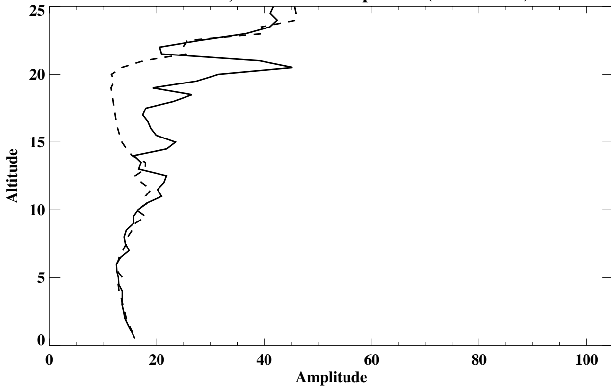
Paramaribo, Suriname' Amplitude (% of mean)
