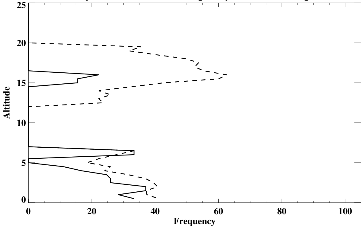
Alajuela, Costa Rica Frequency (% of soundings)
