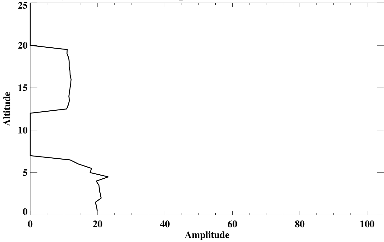
Alajuela, Costa Rica Amplitude (% of mean) (Total Lamina)
