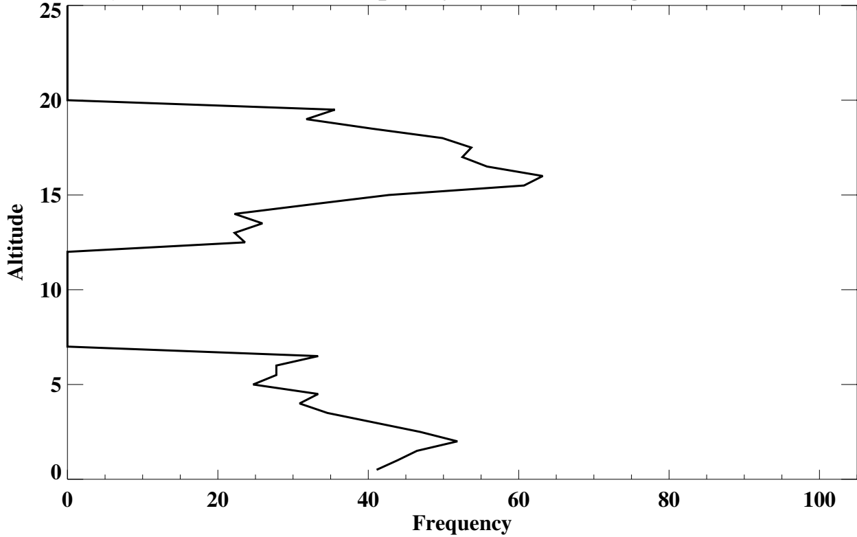
Alajuela, Costa Rica Frequency (% of soundings) (Total Lamina)
