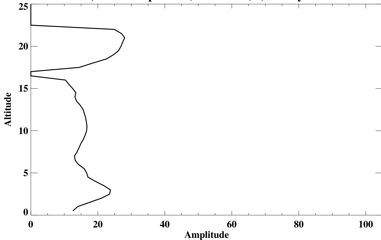
Yellowknife, NWT Amplitude (% of mean) (Gravity Wave Lamina)
