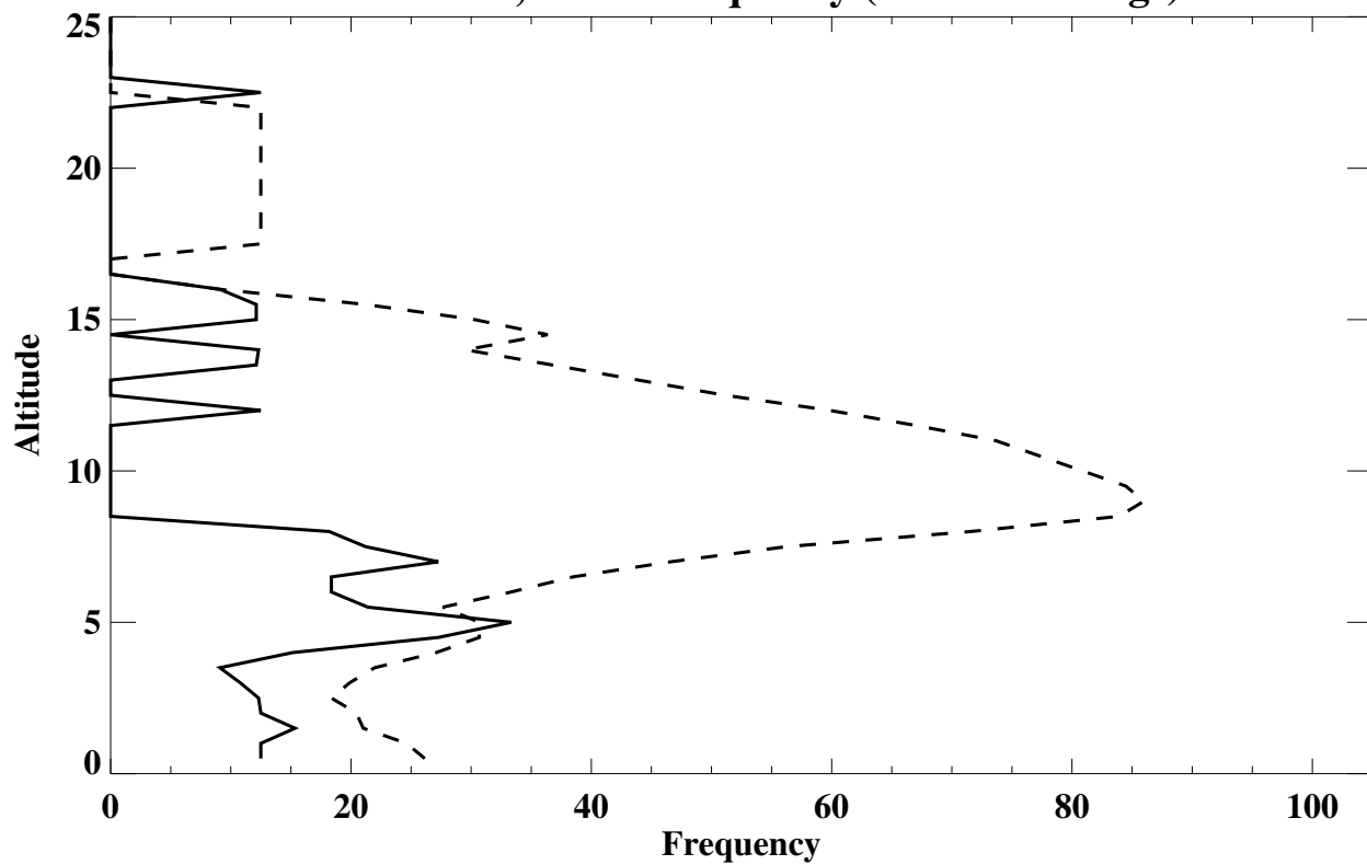
Yellowknife, NWT Frequency (% of soundings)
