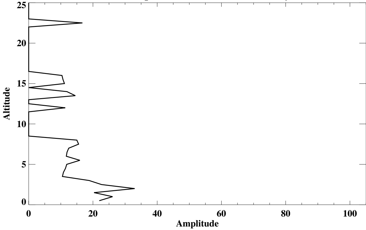
Yellowknife, NWT Amplitude (% of mean) (Rossby wave Lamina)
