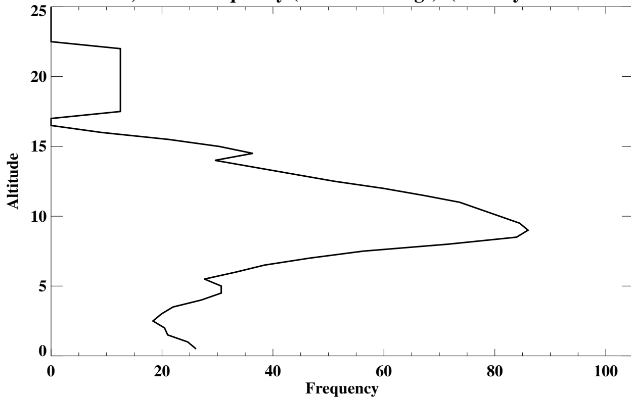
Yellowknife, NWT Frequency (% of soundings) (Gravity Wave Lamina)
