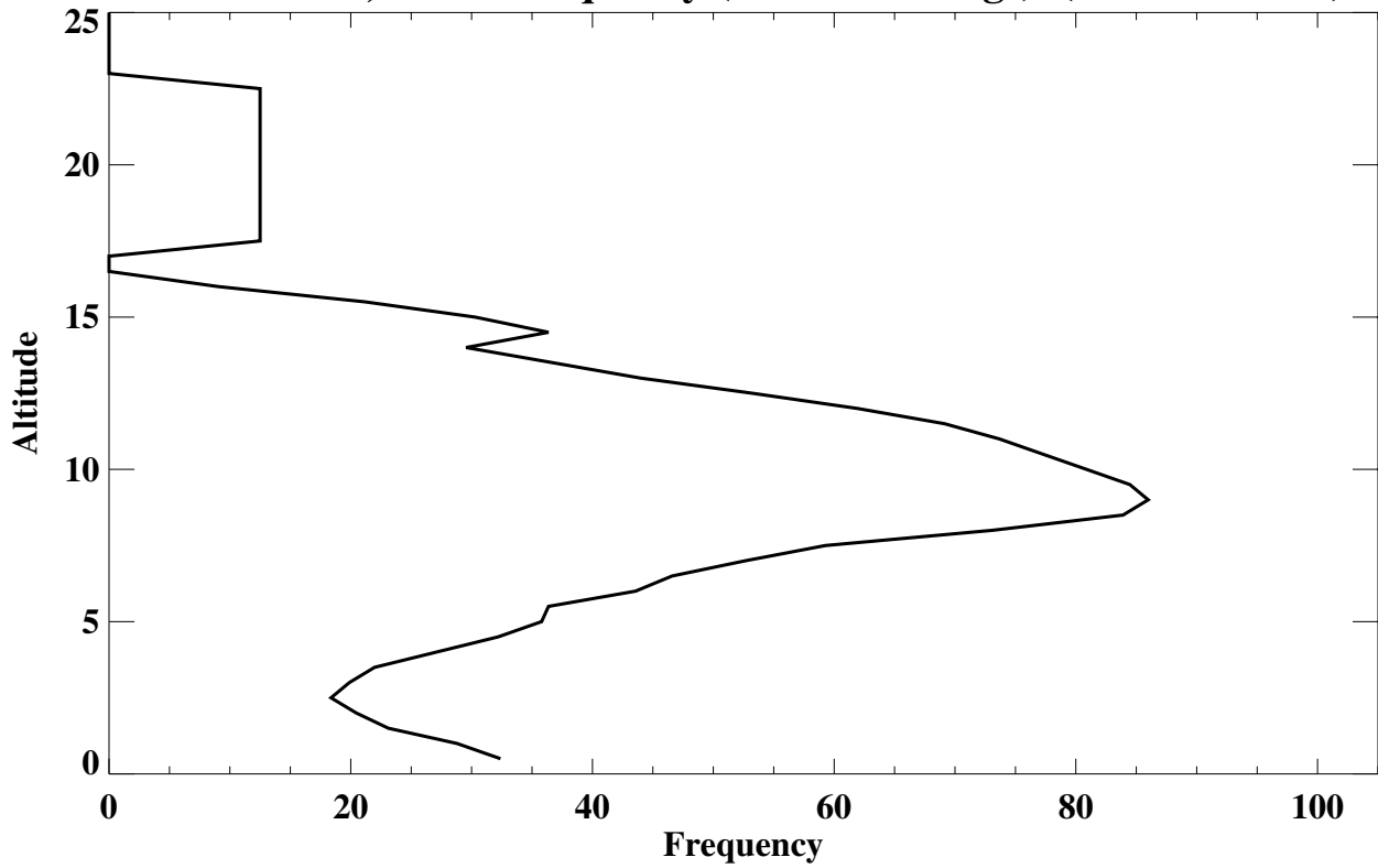
Yellowknife, NWT Frequency (% of soundings) (Total Lamina)
