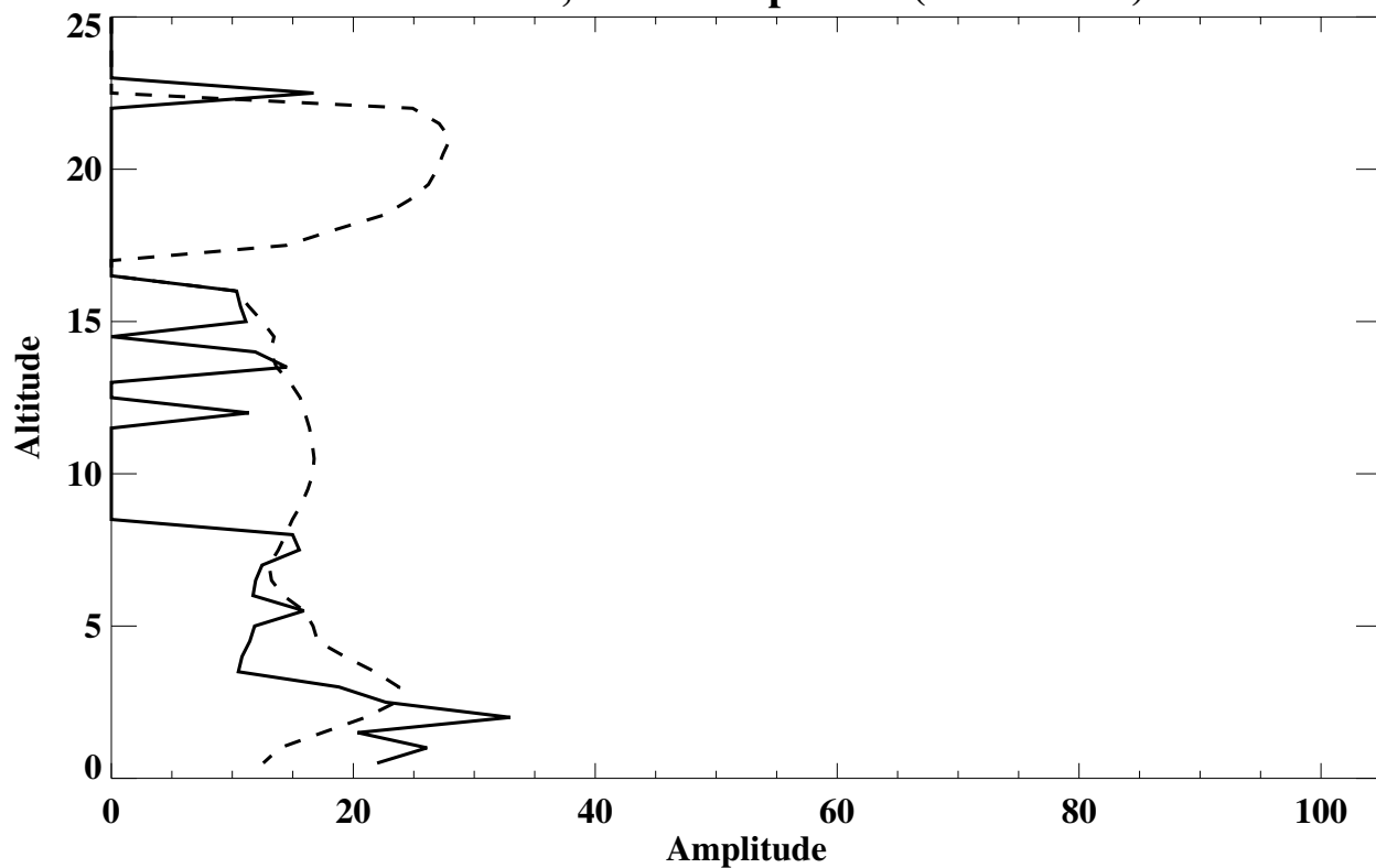
Yellowknife, NWT Amplitude (% of mean)
