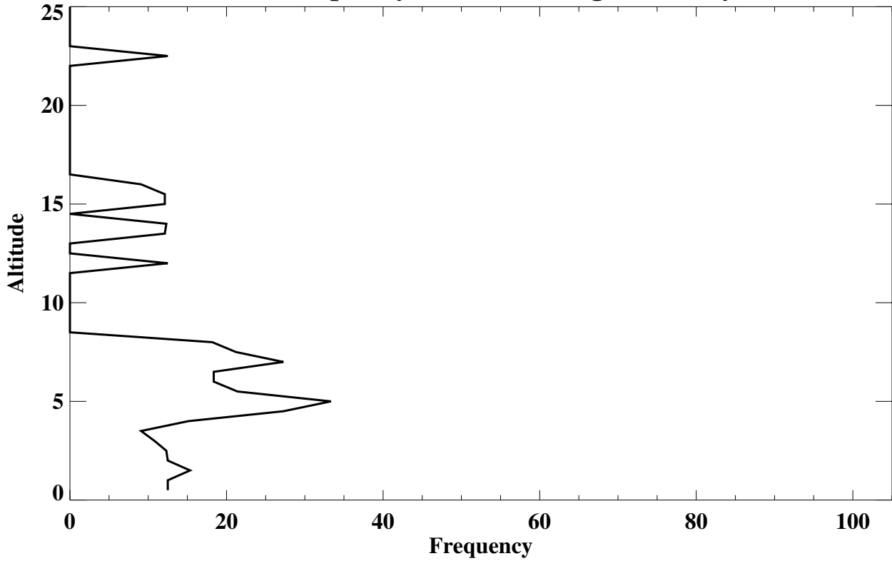
Yellowknife, NWT Frequency (% of soundings) (Rossby wave Lamina)
