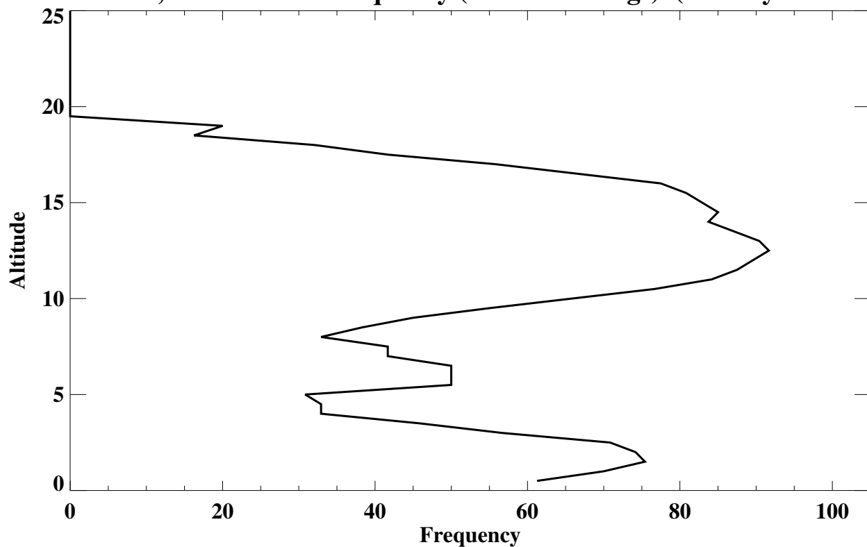
Trinidad Head, CA Lamina Frequency (% of soundings) (Gravity Wave Lamina)
