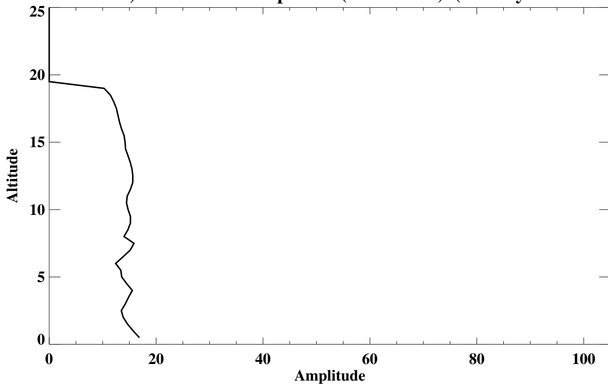
Trinidad Head, CA Lamina Amplitude (% of mean) (Gravity Wave Lamina)
