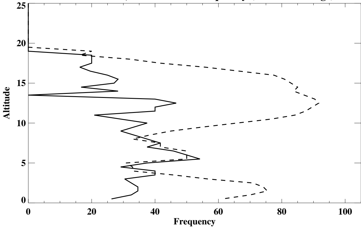
Trinidad Head, CA Lamina Frequency (% of soundings)
