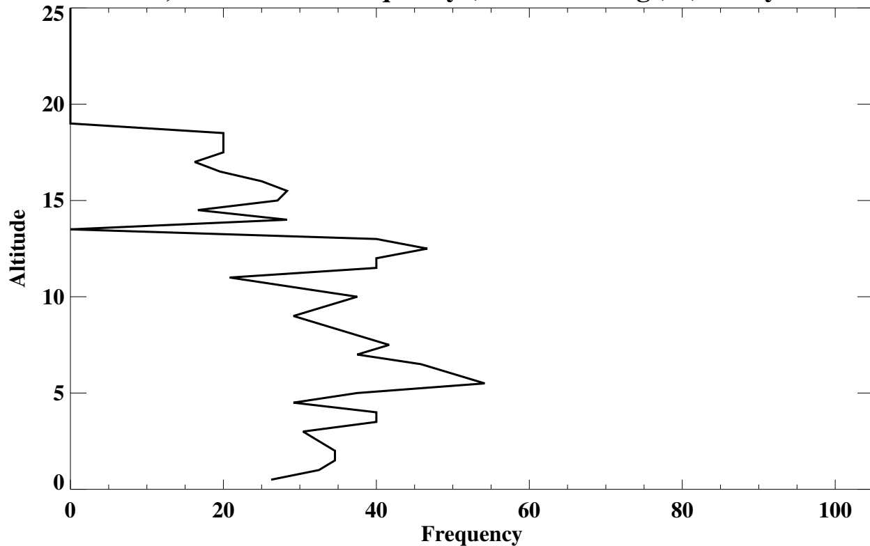
Trinidad Head, CA Lamina Frequency (% of soundings) (Rossby wave Lamina)
