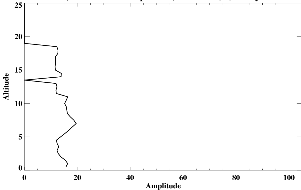
Trinidad Head, CA Lamina Amplitude (% of mean) (Rossby wave Lamina)
