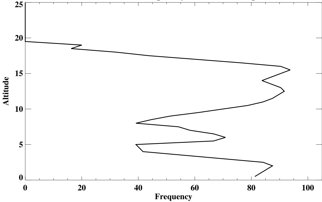
Trinidad Head, CA Lamina Frequency (% of soundings) (Total Lamina)
