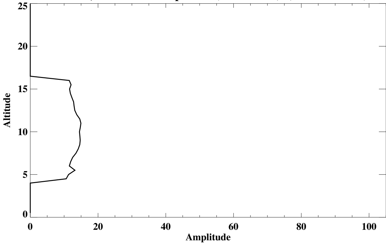
Summit, Greenland Frequency (% of soundings) (Total Lamina)
