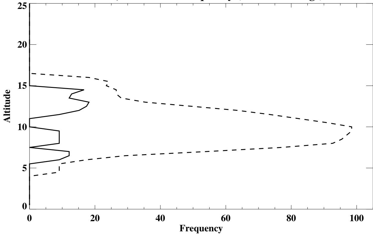
Summit, Greenland Frequency (% of soundings)
