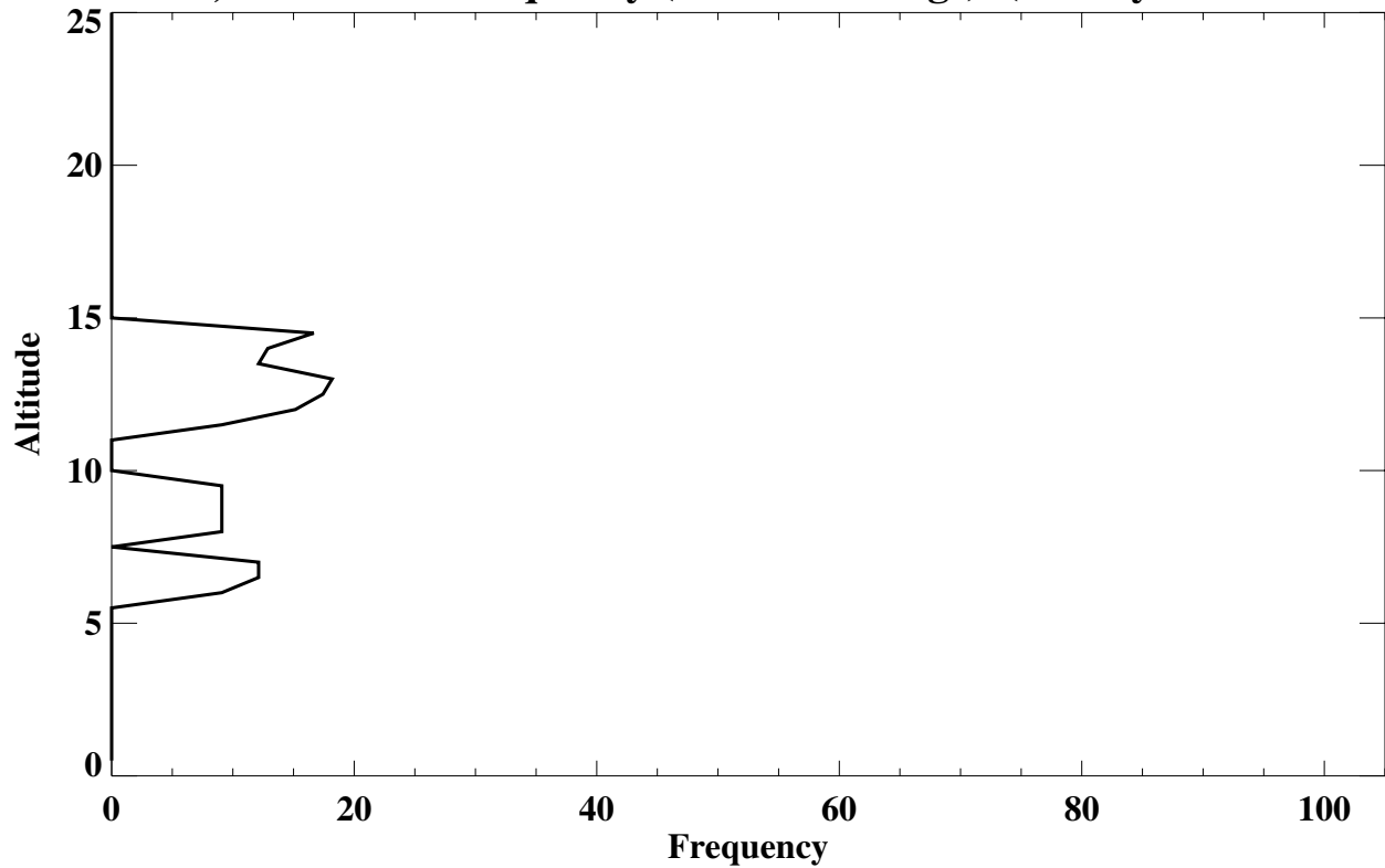
Summit, Greenland Frequency (% of soundings) (Rossby wave Lamina)
