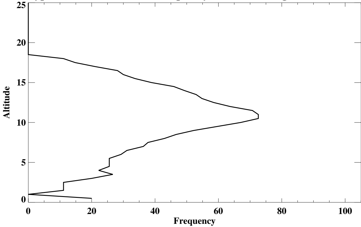
Stonyplain, Alberta Lamina Frequency (% of soundings) (Total Lamina)
