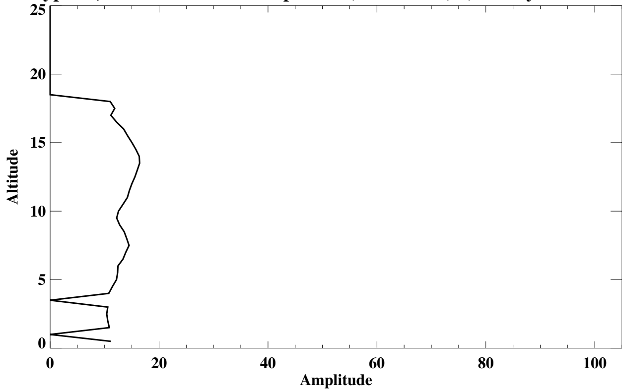
Stonyplain, Alberta Lamina Frequency (% of soundings) (Gravity Wave Lamina)
