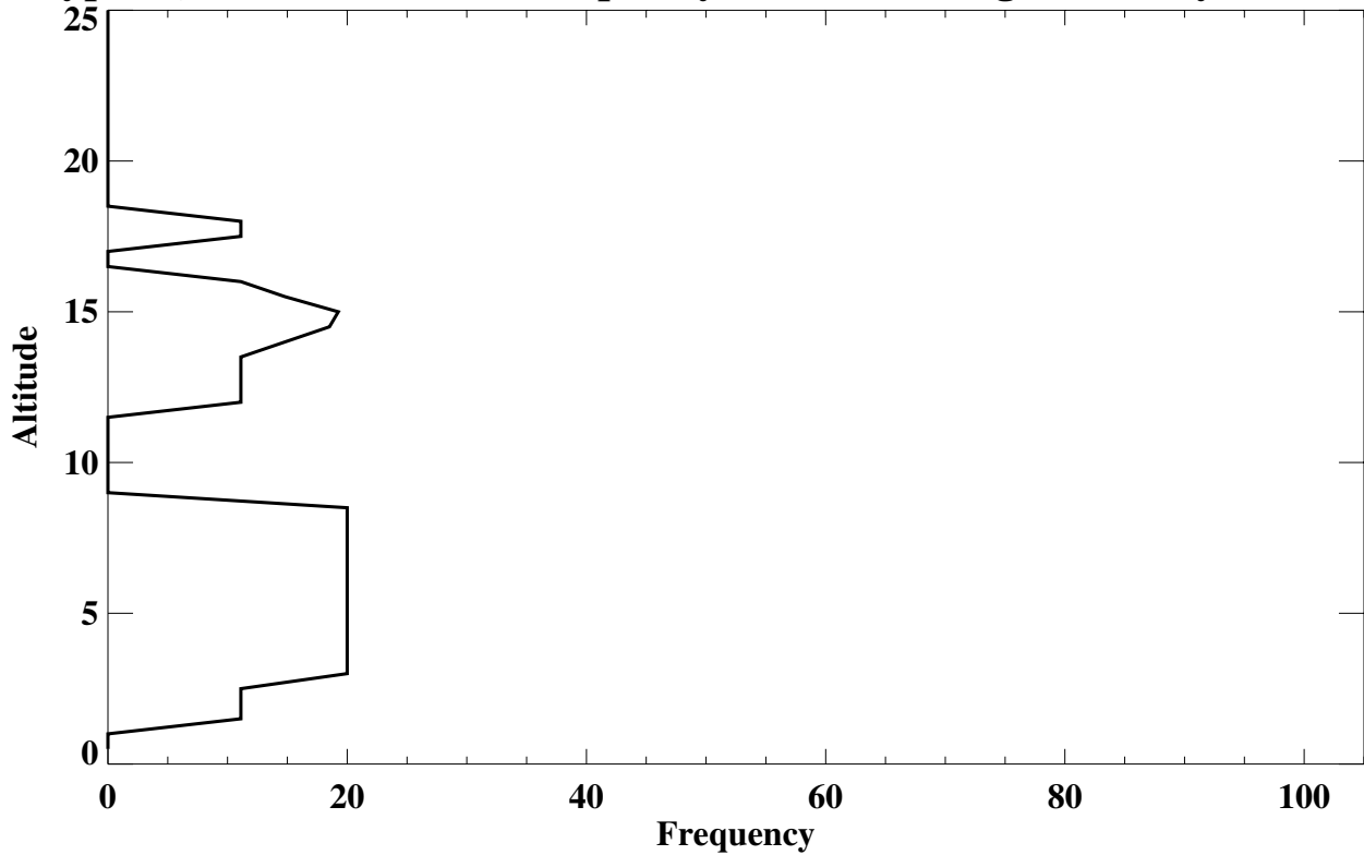
Stonyplain, Alberta Lamina Frequency (% of soundings) (Rossby wave Lamina)
