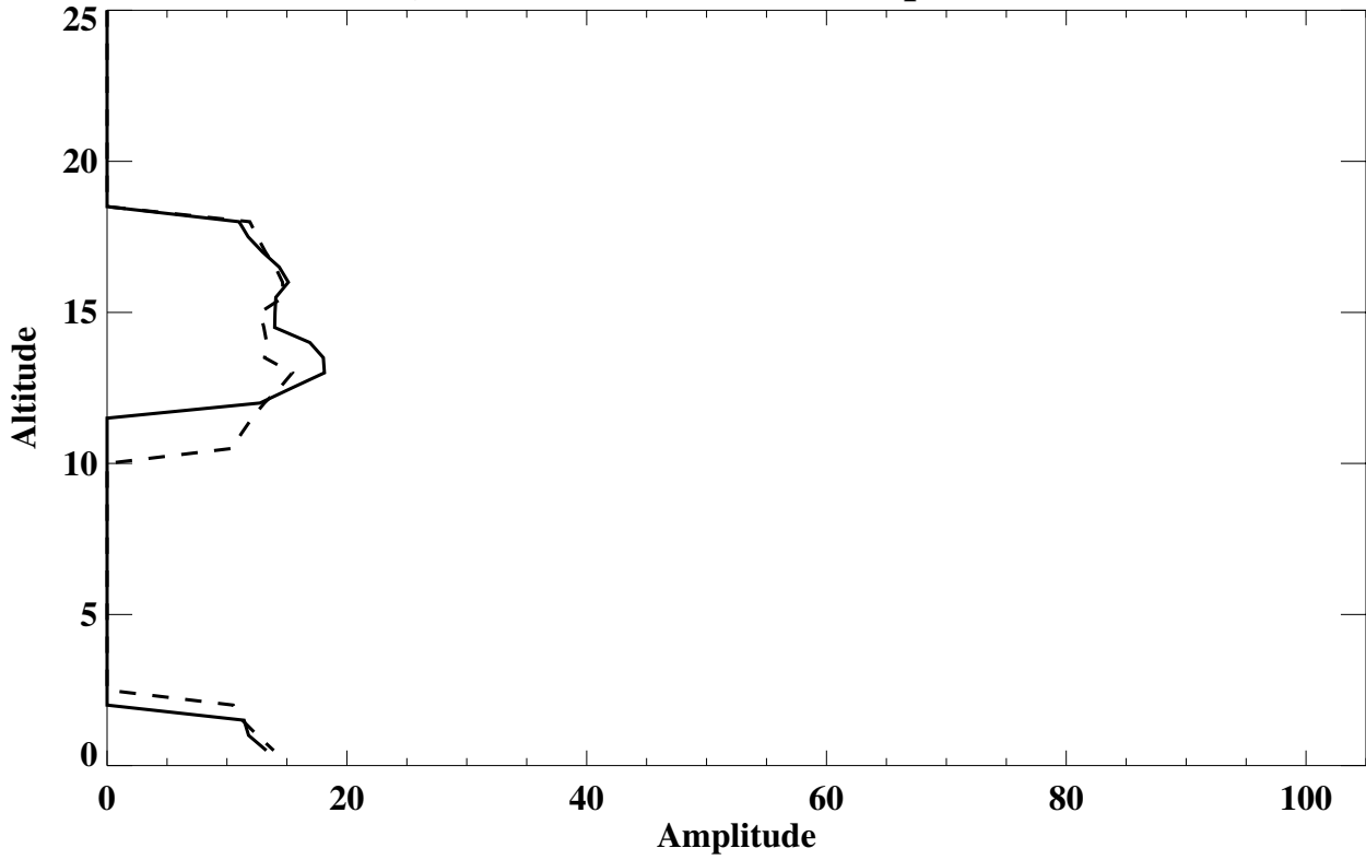
Sable Island, Nova Scotia Lamina Amplitude (% of mean)
