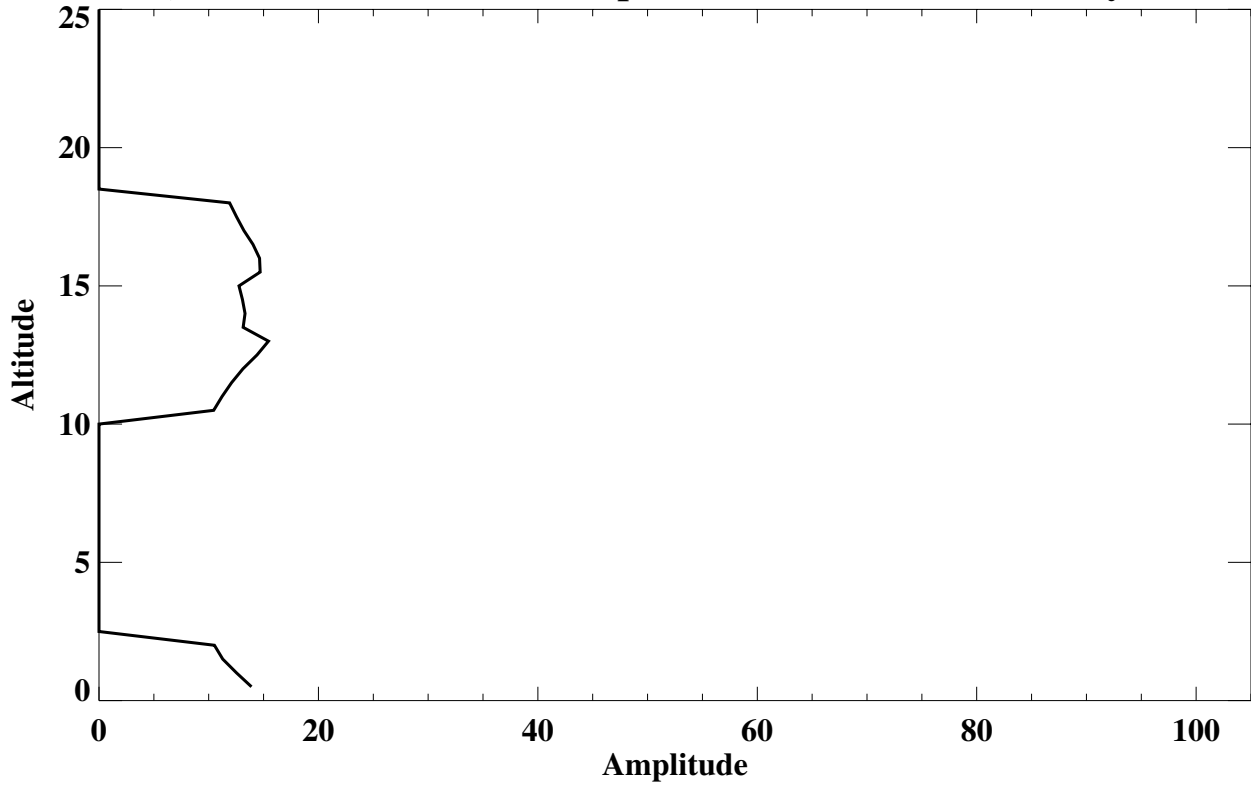
Sable Island, Nova Scotia Lamina Amplitude (% of mean) (Gravity Wave Lamina)
