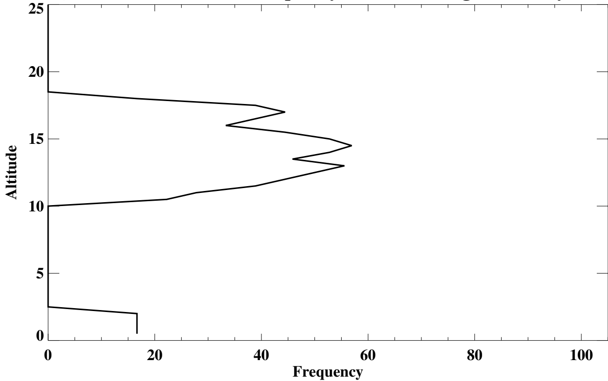
Sable Island, Nova Scotia Lamina Frequency (% of soundings) (Gravity Wave Lamina)
