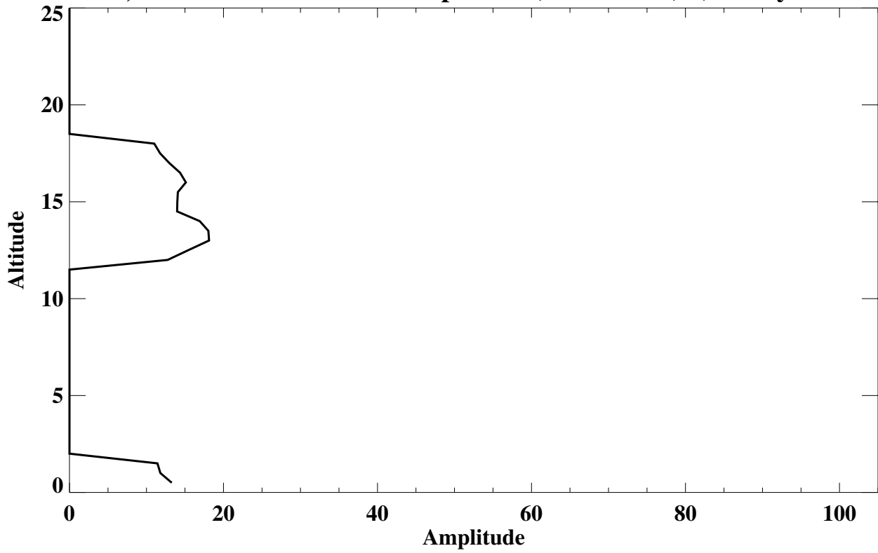
Sable Island, Nova Scotia Lamina Frequency (% of soundings) (Rossby wave Lamina)
