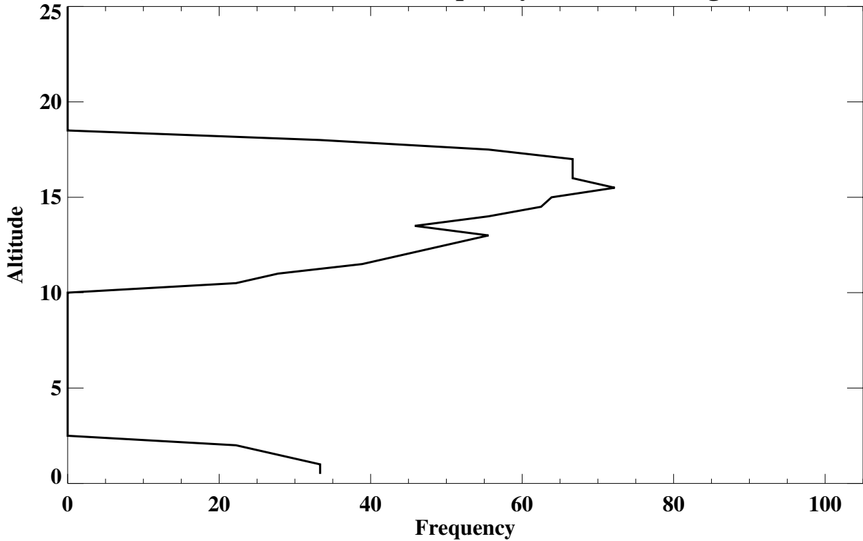
Sable Island, Nova Scotia Lamina Frequency (% of soundings) (Total Lamina)
