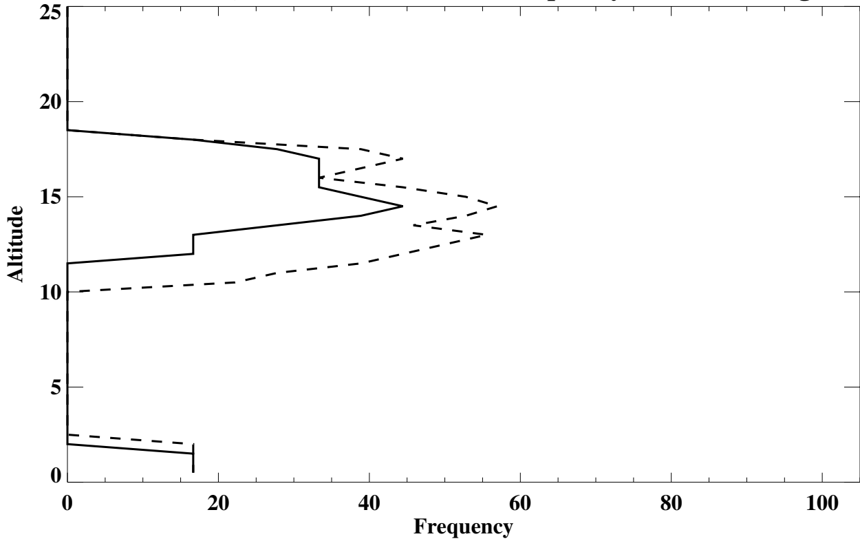
Sable Island, Nova Scotia Lamina Frequency (% of soundings)
