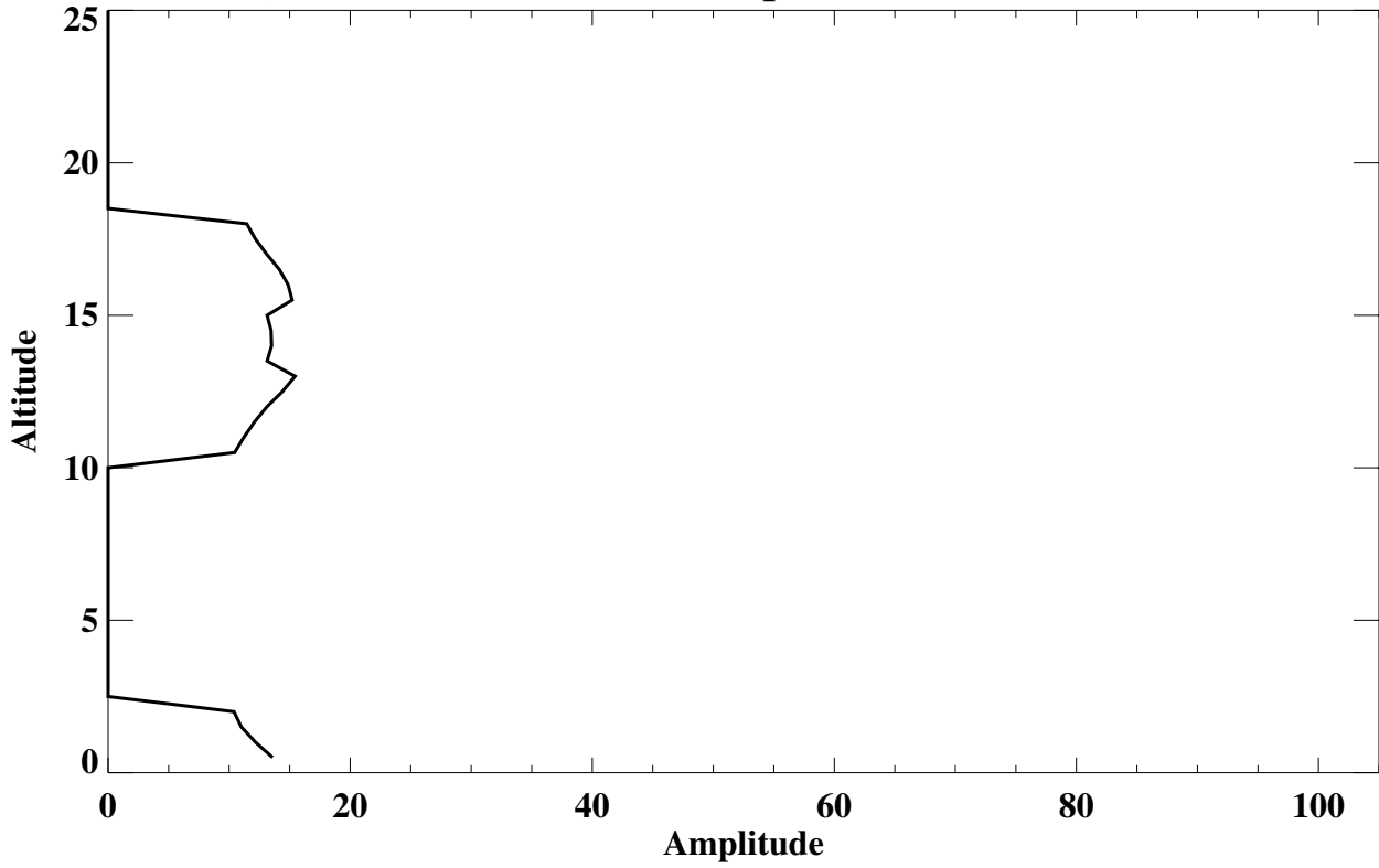
Sable Island, Nova Scotia Lamina Amplitude (% of mean) (Total Lamina)
