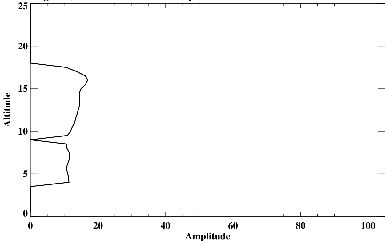
Egbert, Ontario Lamina Frequency (% of soundings) (Total Lamina)
