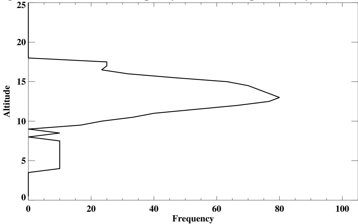
Egbert, Ontario Lamina Frequency (% of soundings) (Gravity Wave Lamina)
