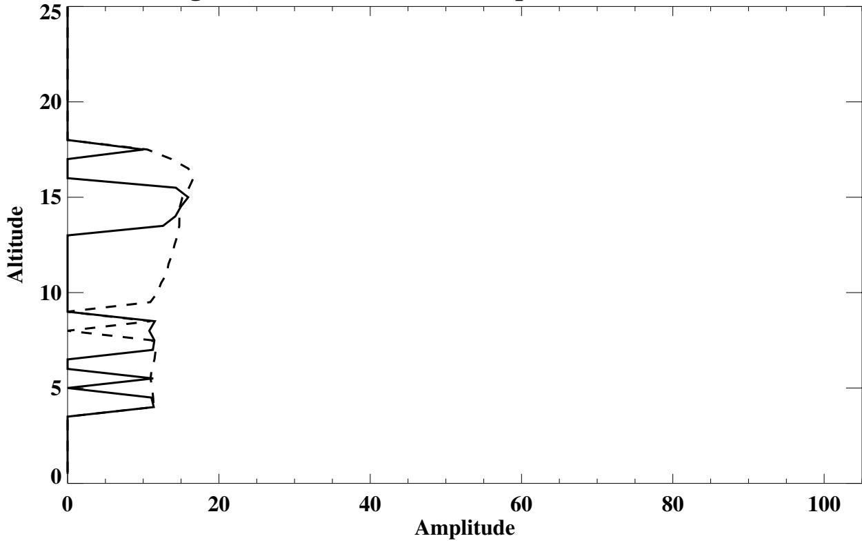
Egbert, Ontario Lamina Frequency (% of soundings)
