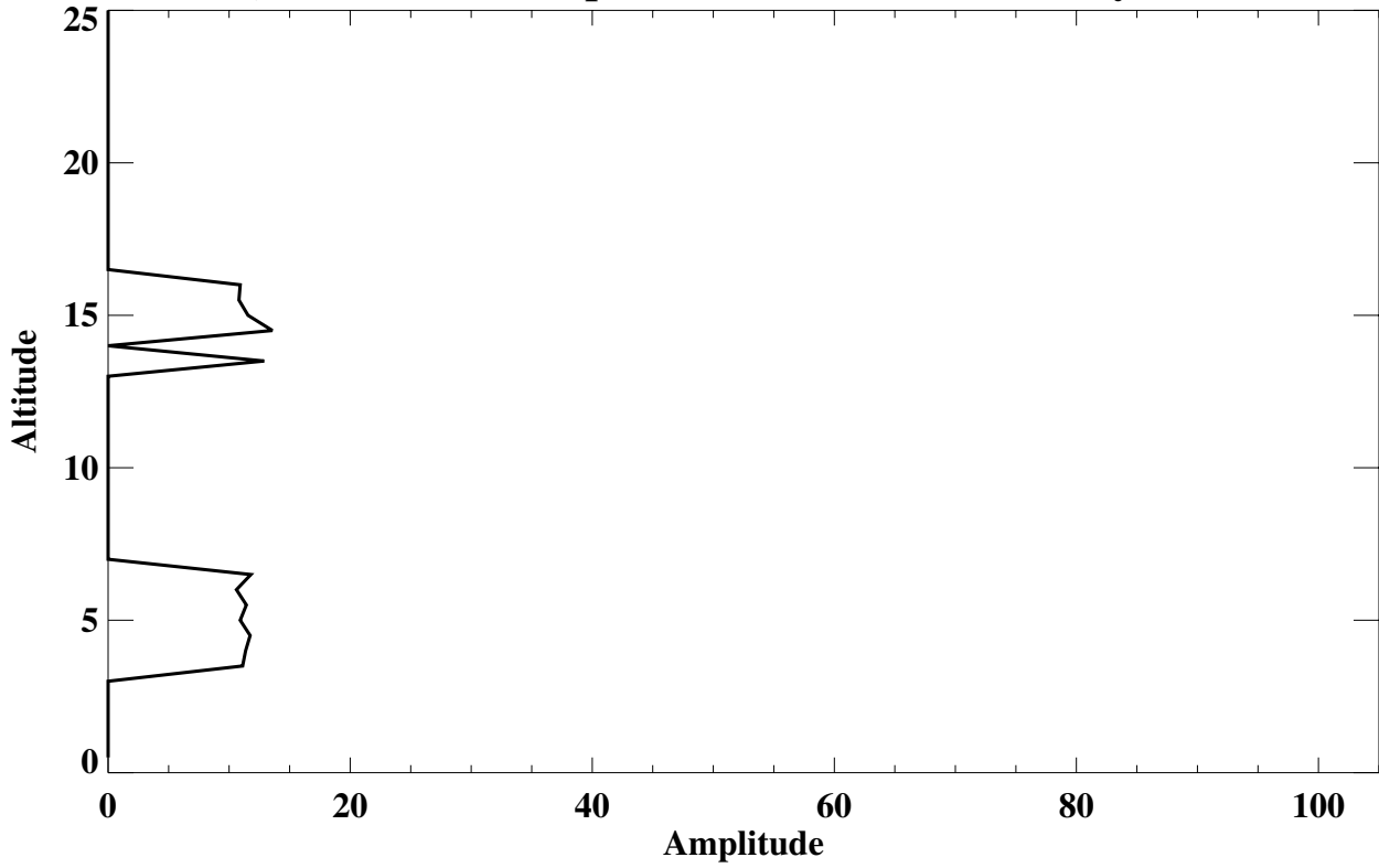
Churchill, MB Lamina Amplitude (% of mean) (Rossby wave Lamina)
