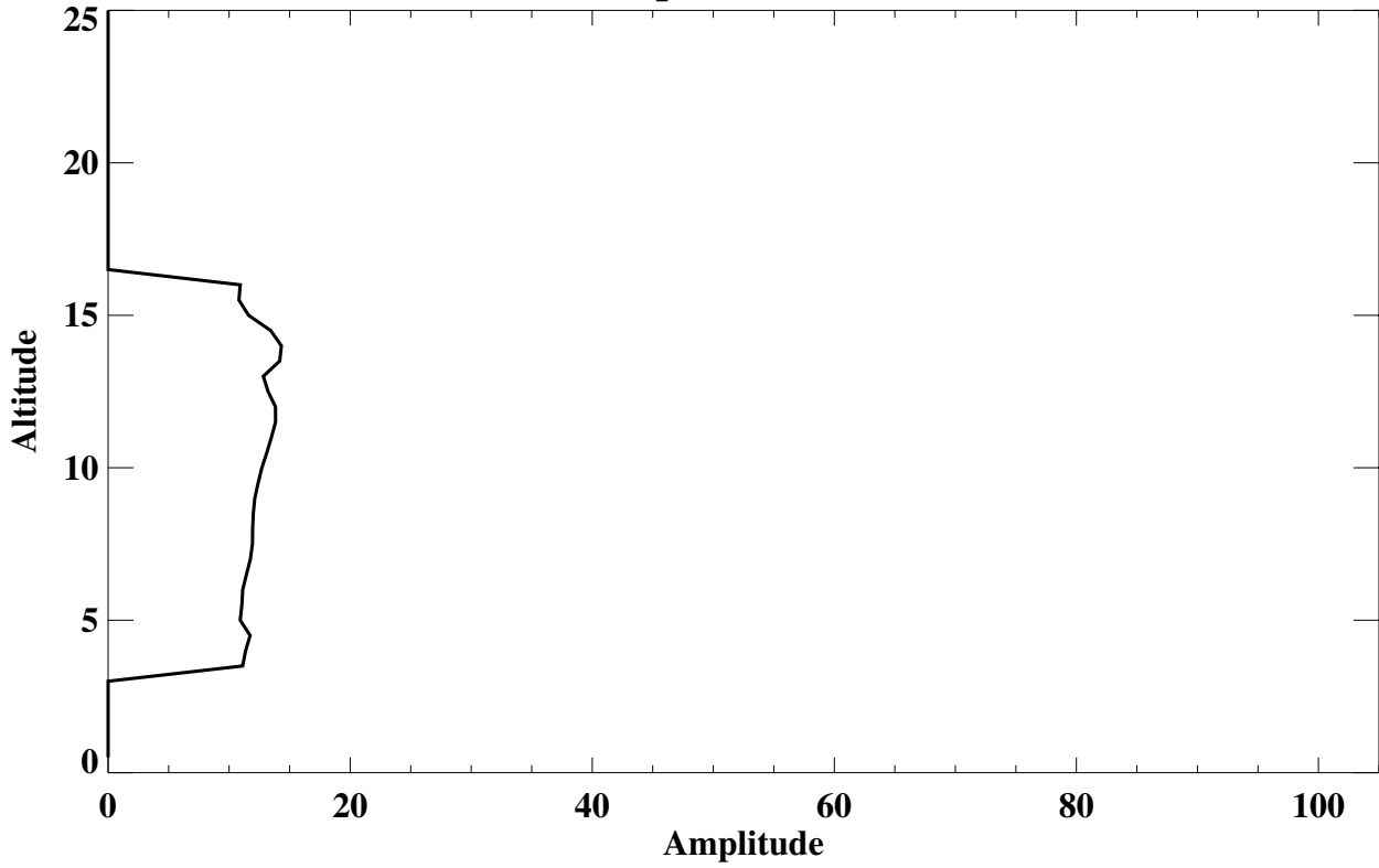
Churchill, MB Lamina Frequency (% of soundings) (Total Lamina)
