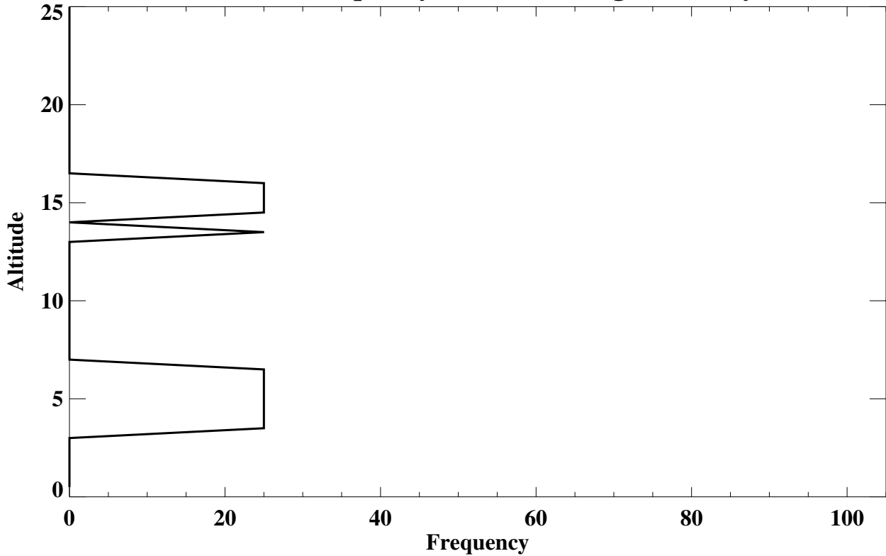
Churchill, MB Lamina Frequency (% of soundings) (Rossby wave Lamina)
