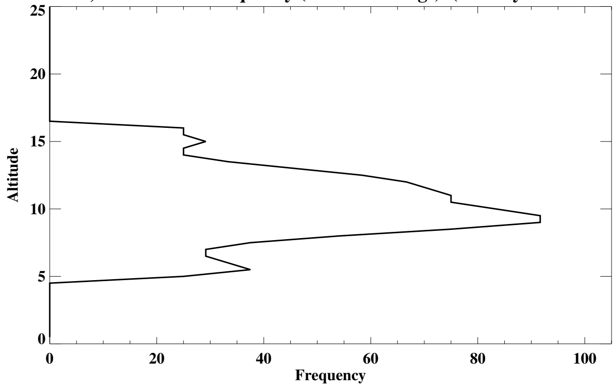
Churchill, MB Lamina Frequency (% of soundings) (Gravity Wave Lamina)
