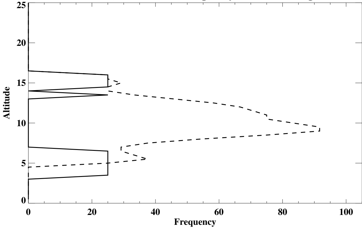
Churchill, MB Lamina Frequency (% of soundings)
