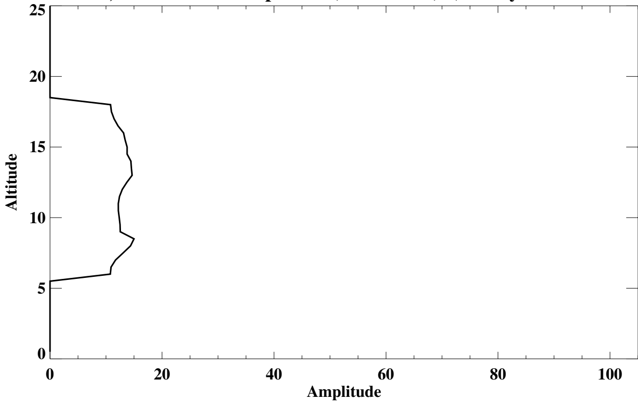
Boulder, CO Lamina Frequency (% of soundings) (Rossby wave Lamina)
