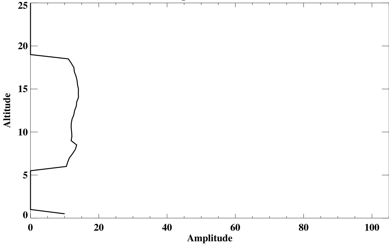
Boulder, CO Lamina Amplitude (% of mean) (Total Lamina)
