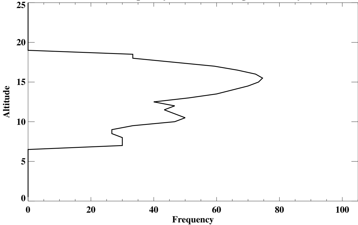
Boulder, CO Lamina Frequency (% of soundings) (Gravity Wave Lamina)
