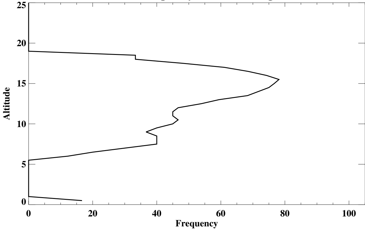
Boulder, CO Lamina Frequency (% of soundings) (Total Lamina)
