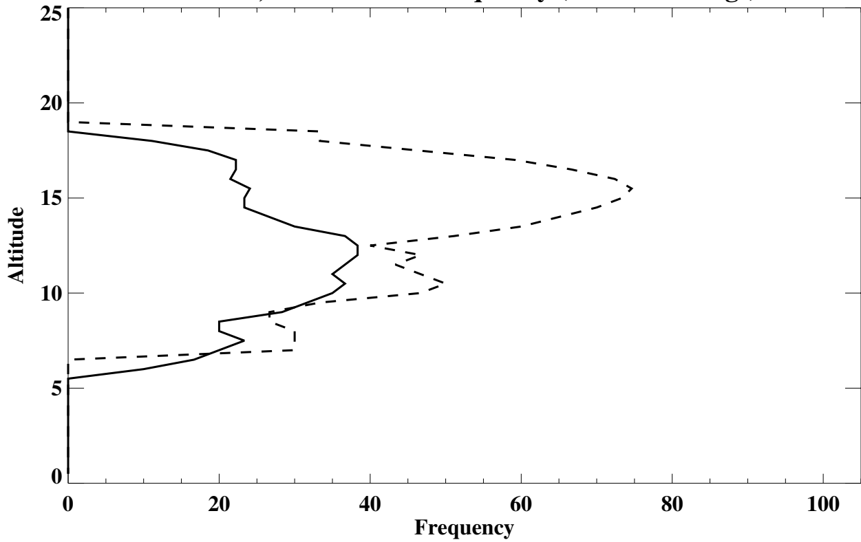
Boulder, CO Lamina Frequency (% of soundings)
